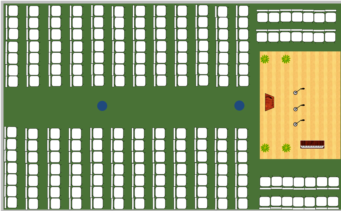
30' X 50' auditorium seating floor plan
